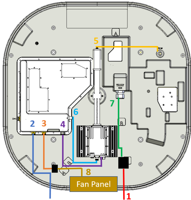
u8 Terminal Cabling Diagram
