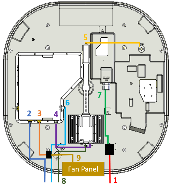
u8 ODU Cabling Diagram
