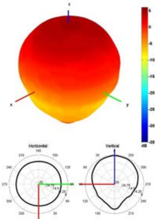
1621 MHz Radiation pattern
